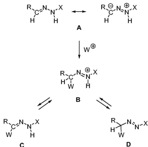
Scheme 4
