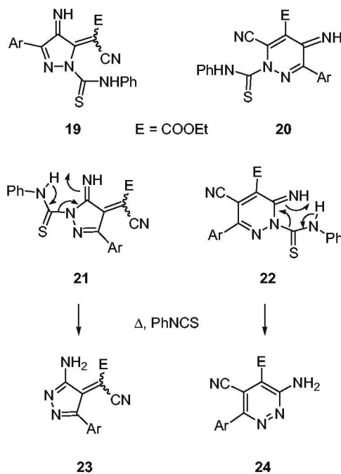
Scheme 7
