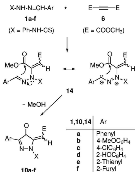
Scheme 6
