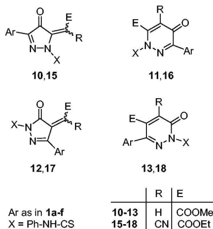
Scheme 5
